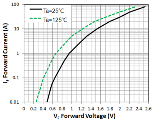
Figure 1. Forward Characteristic(typ.)
