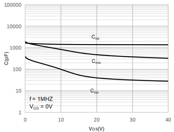
Figure 6: Capacitance Characteristics
